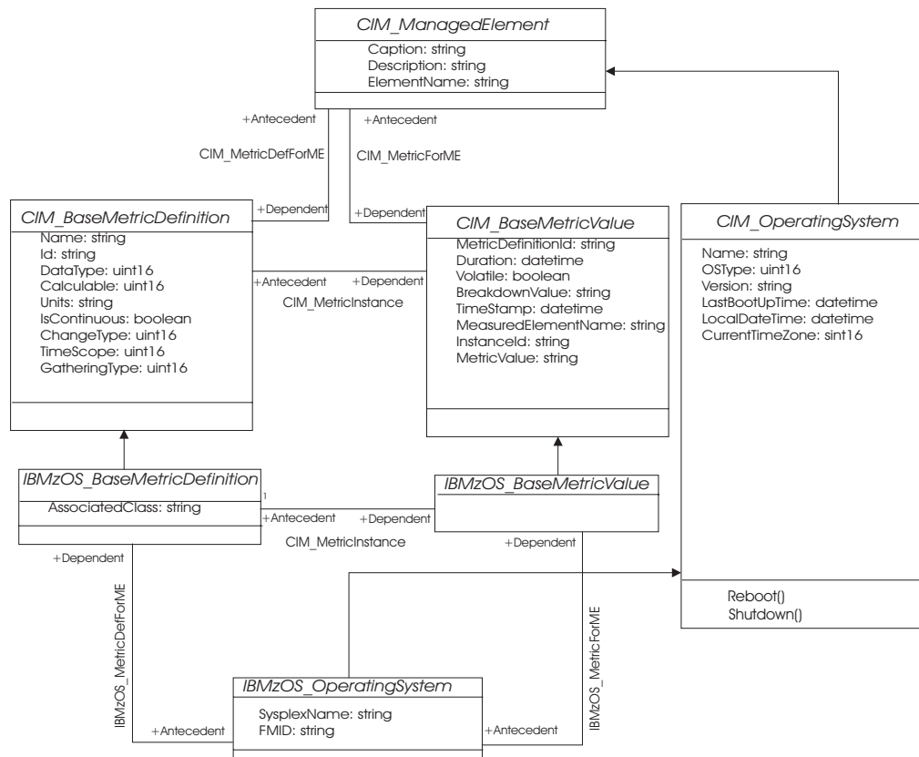
Figure 8. z/OS RMF implementation of the DMTF dynamic metrics model
