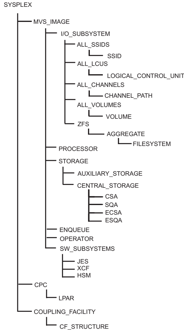
Figure 7. The Monitor III resource model
