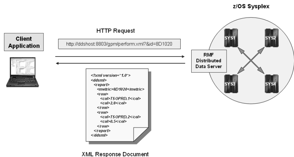
Figure 6. How to use the DDS HTTP API
